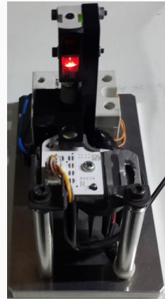
LIGHT GUIDE YAKMA TEST CİHAZI
